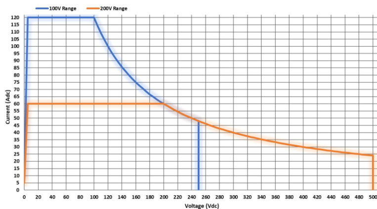
ASR-6600-12 DC Mode Output Operating Area
