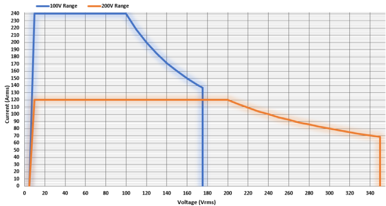
ASR-6600-24 AC Mode Output Operating Area
