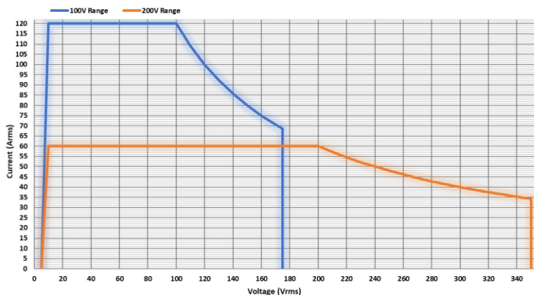
ASR-6600-12 AC Mode Output Operating Area
