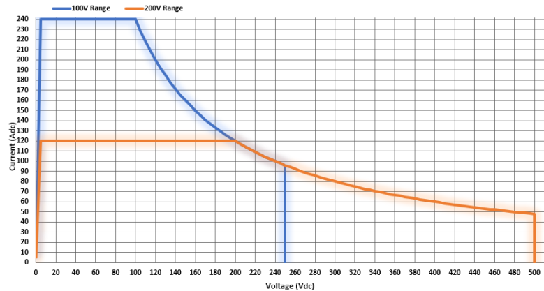
ASR-6600-24 DC Mode Output Operating Area
