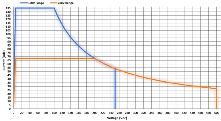
ASR-6450-13.5 DC Mode Output Operating Area
