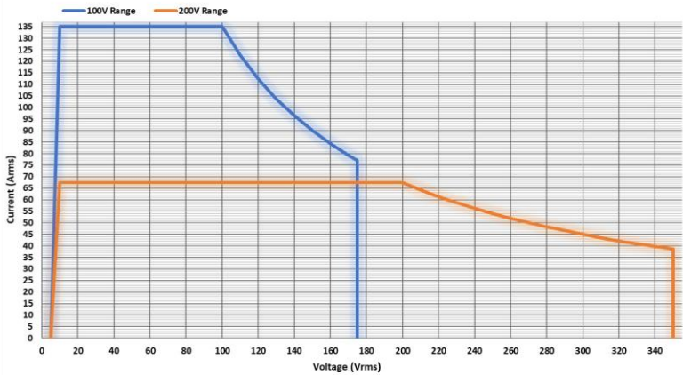
ASR-6450-13.5 AC Mode Output Operating Area
